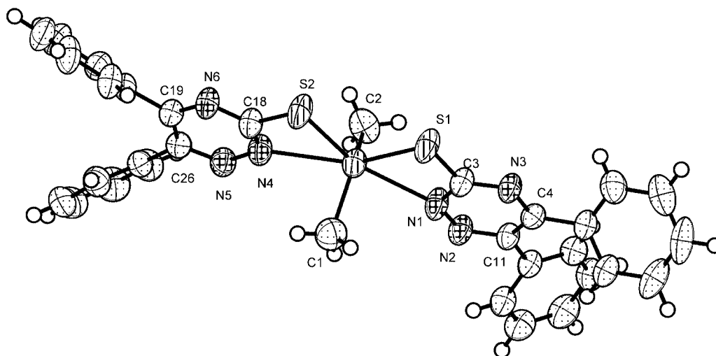
Figure 2. XSHELL view of [\text{SnMe}_2(\text{C}_{15}\text{H}_{10}\text{N}_3\text{S})_2] ( 4 )
