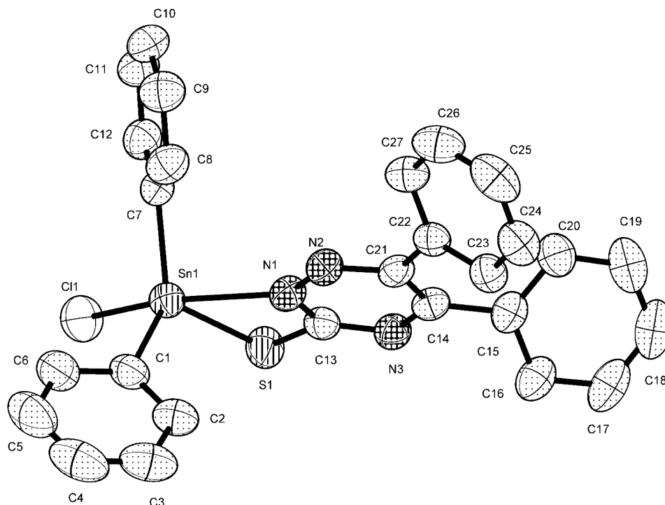
Figure 1. XSEHELL view of [\text{SnPh}_2(\text{C}_{15}\text{H}_{10}\text{N}_3\text{S})\text{Cl}] ( 1 )
